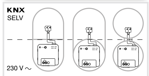
Figure 2: installation with separate terminal compartment
