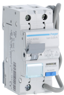
ADA925U
