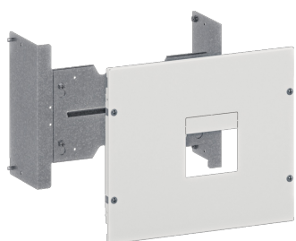
UC233PN
